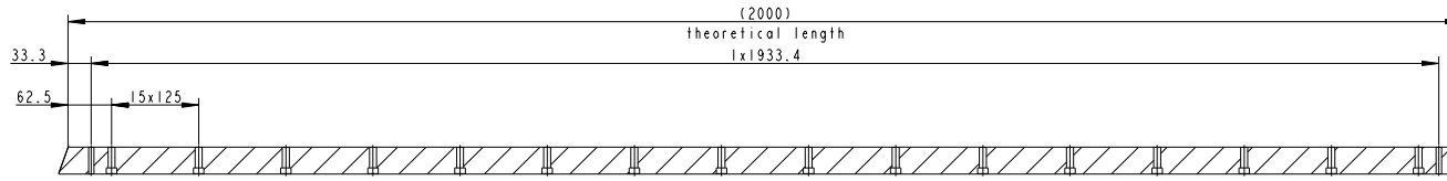
SECTION C-C
