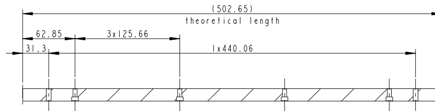
SECTION C-C
